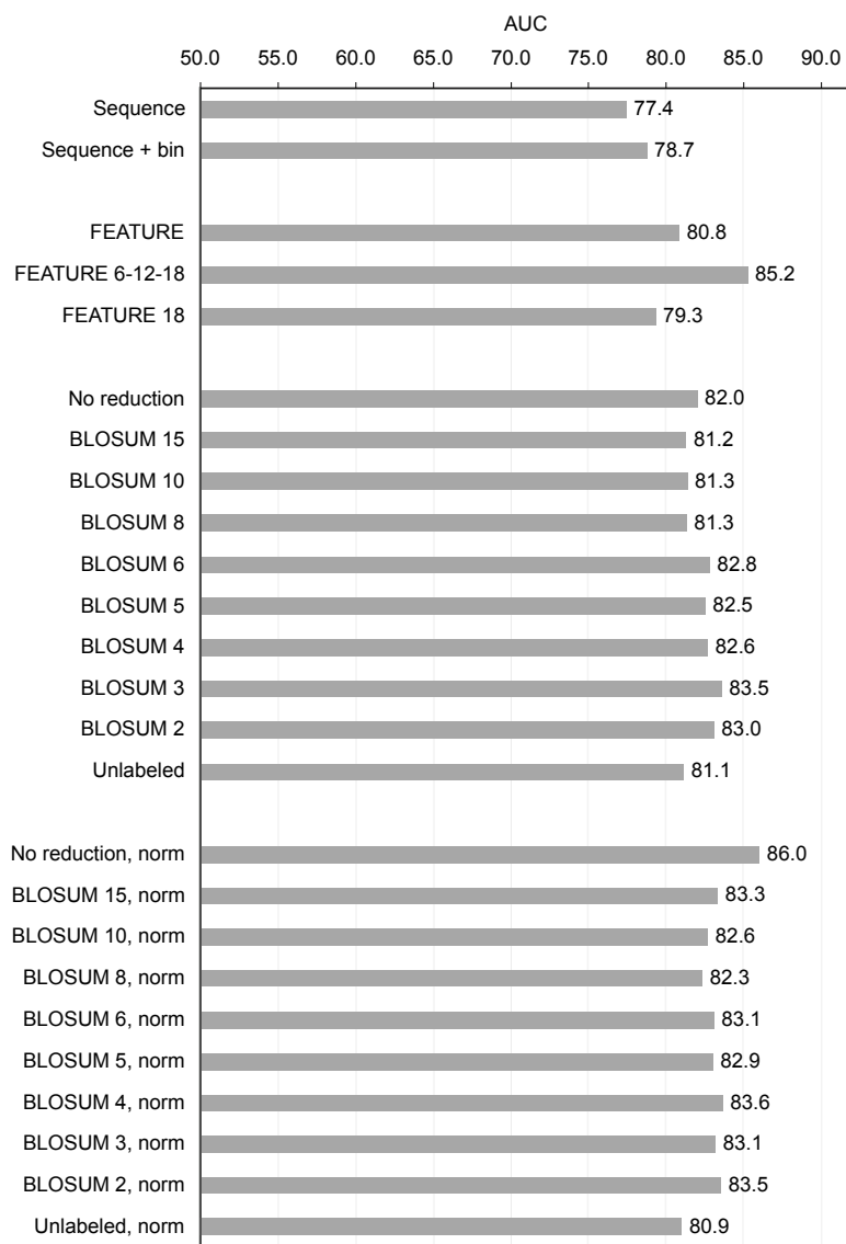
Supplementary Figure S13: Performance of all predictors on the CSA-Lys dataset.
