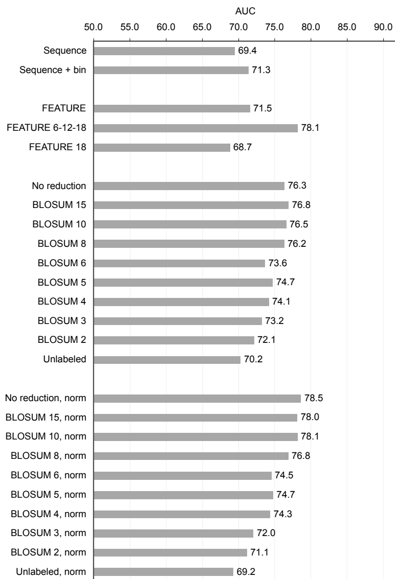
Supplementary Figure S10: Performance of all predictors on the CSA-His dataset.
