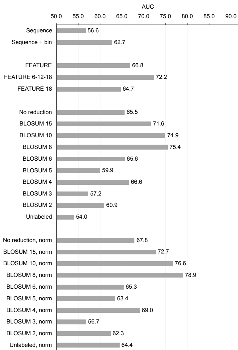
Supplementary Figure S21: Performance of all predictors on the CSA-Val dataset.
