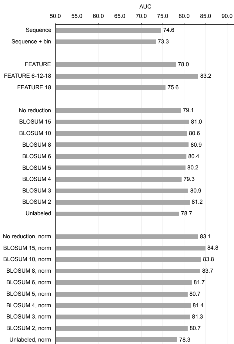
Supplementary Figure S8: Performance of all predictors on the CSA-Glu dataset.
