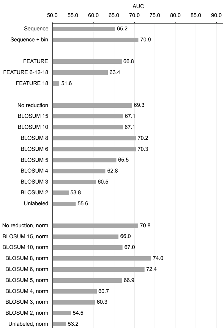
Supplementary Figure S16: Performance of all predictors on the CSA-Pro dataset.
