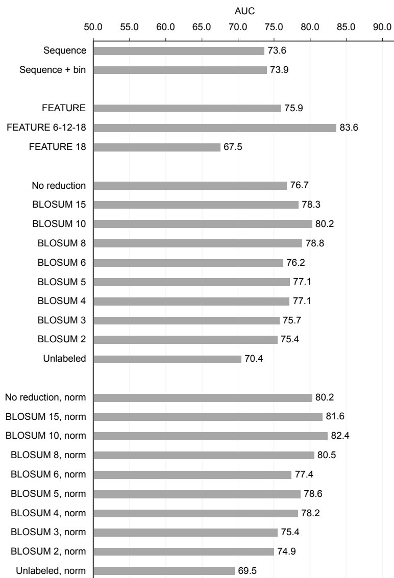
Supplementary Figure S18: Performance of all predictors on the CSA-Thr dataset.
