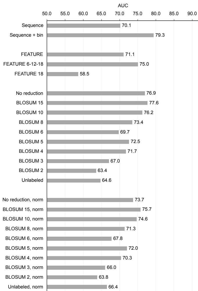
Supplementary Figure S12: Performance of all predictors on the CSA-Leu dataset.
