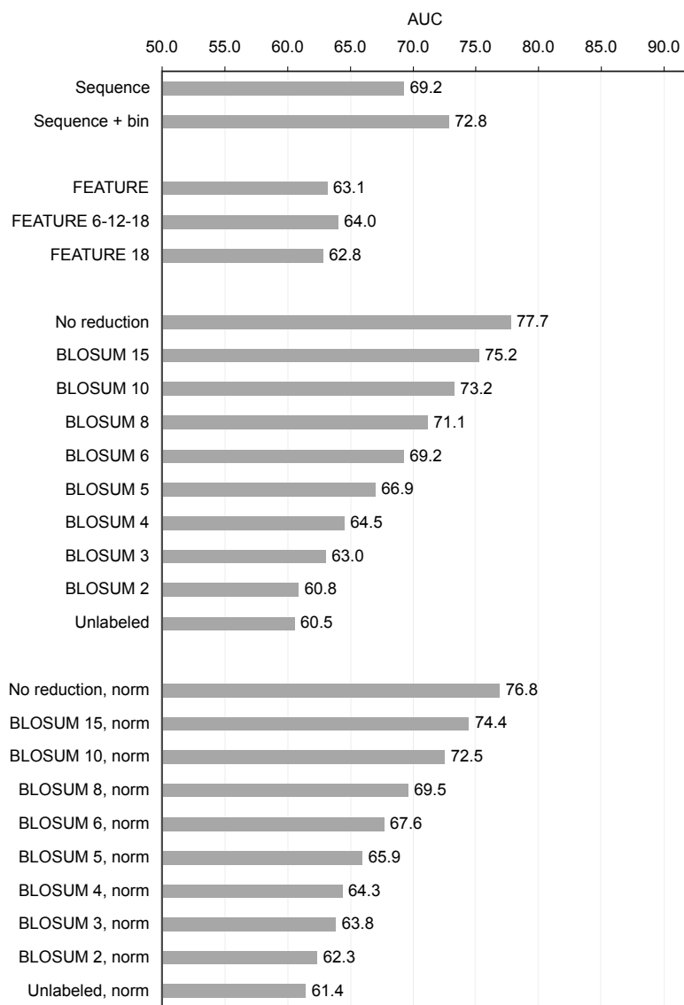
Supplementary Figure S22: Performance of all predictors on the PHOS-Ser dataset.
