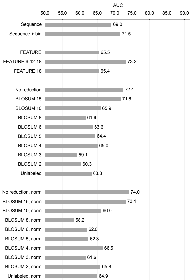
Supplementary Figure S19: Performance of all predictors on the CSA-Trp dataset.
