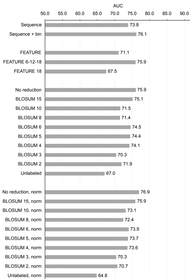
Supplementary Figure S20: Performance of all predictors on the CSA-Tyr dataset.
