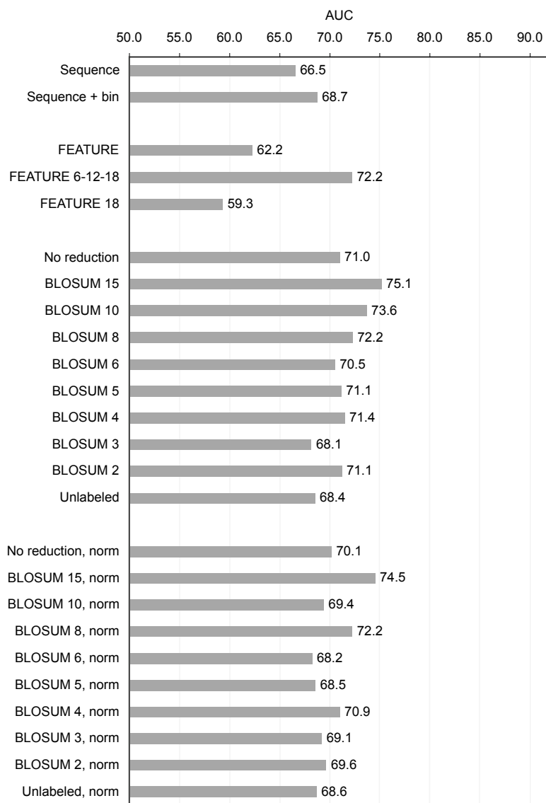
Supplementary Figure S15: Performance of all predictors on the CSA-Phe dataset.
