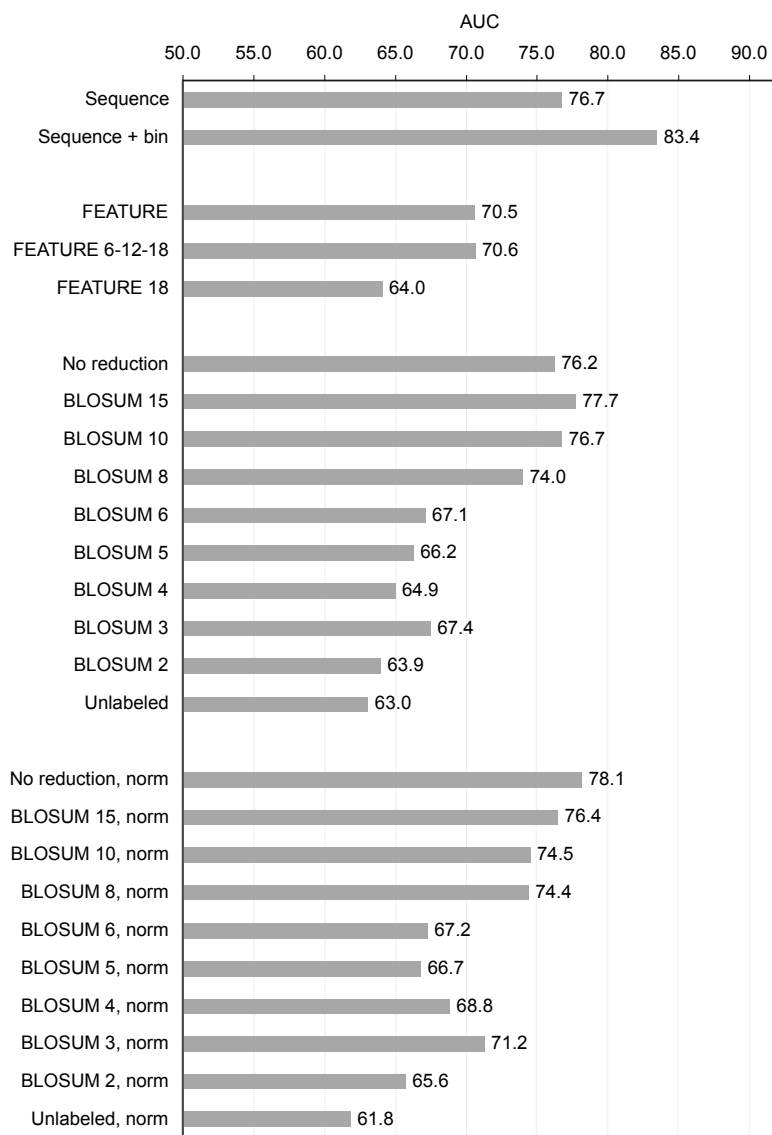
Supplementary Figure S11: Performance of all predictors on the CSA-Ile dataset.
