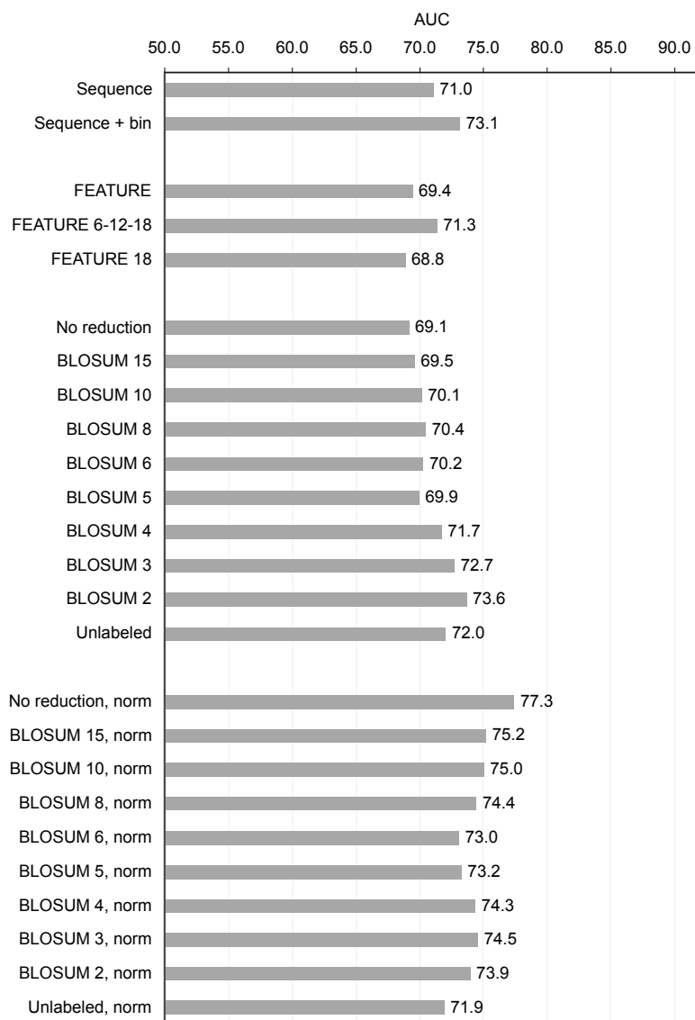
Supplementary Figure S7: Performance of all predictors on the CSA-Gln dataset.
