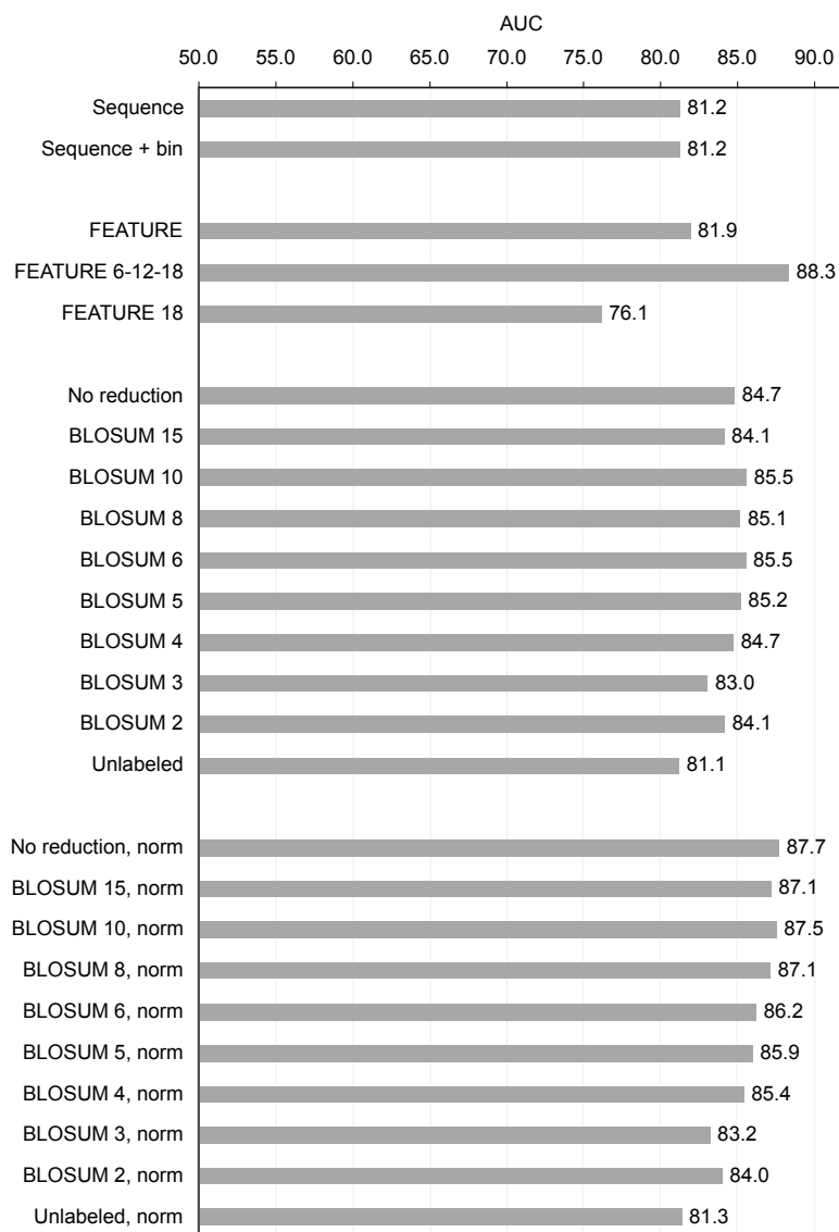
Supplementary Figure S17: Performance of all predictors on the CSA-Ser dataset.
