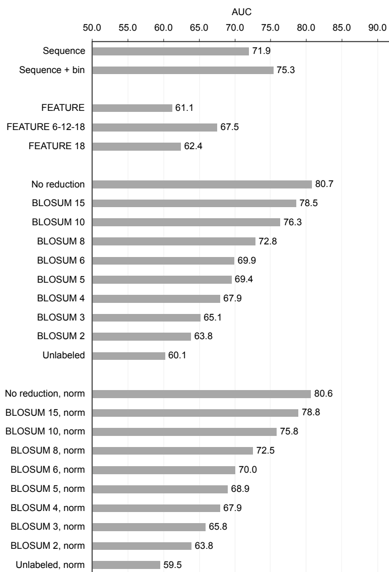
Supplementary Figure S24: Performance of all predictors on the PHOS-Tyr dataset.
