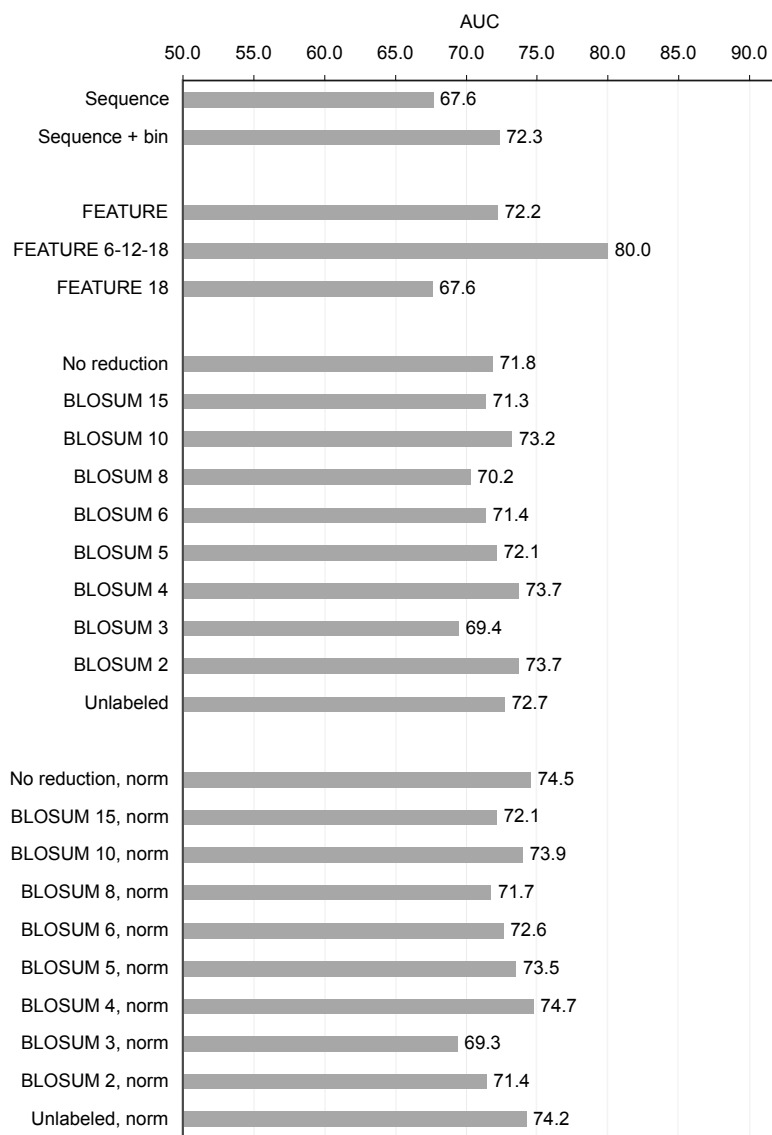
Supplementary Figure S2: Performance of all predictors on the CSA-Ala dataset.
