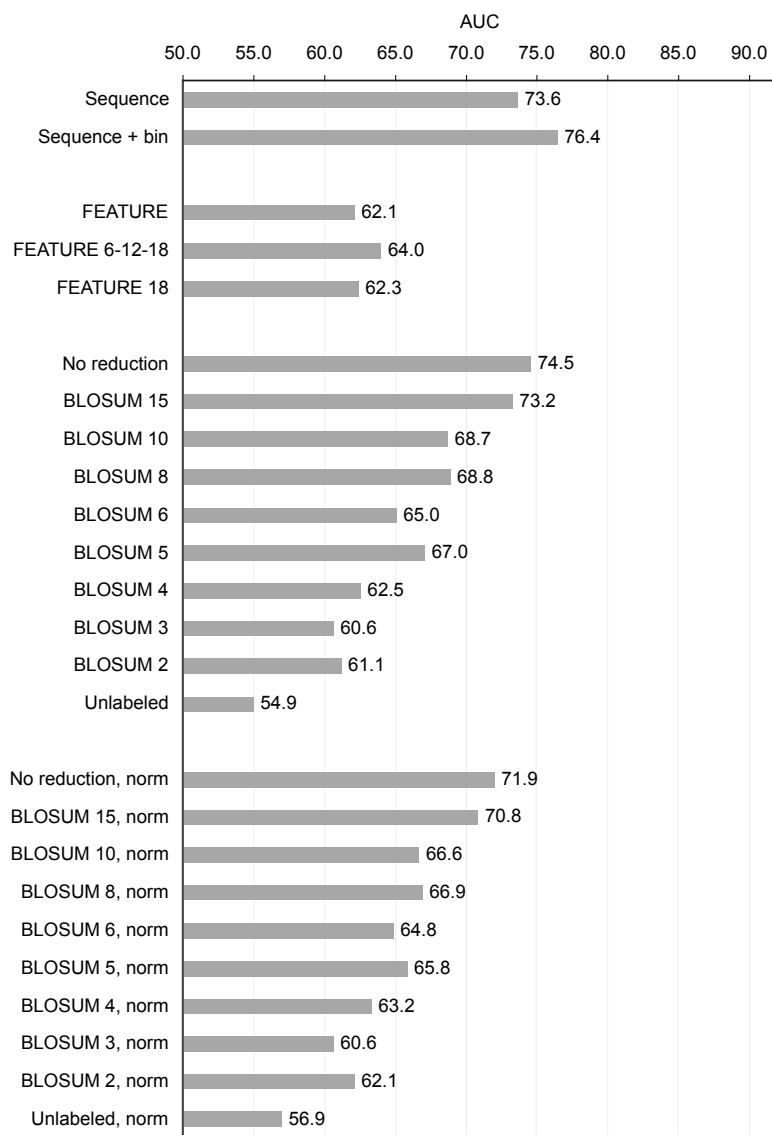
Supplementary Figure S23: Performance of all predictors on the PHOS-Thr dataset.
