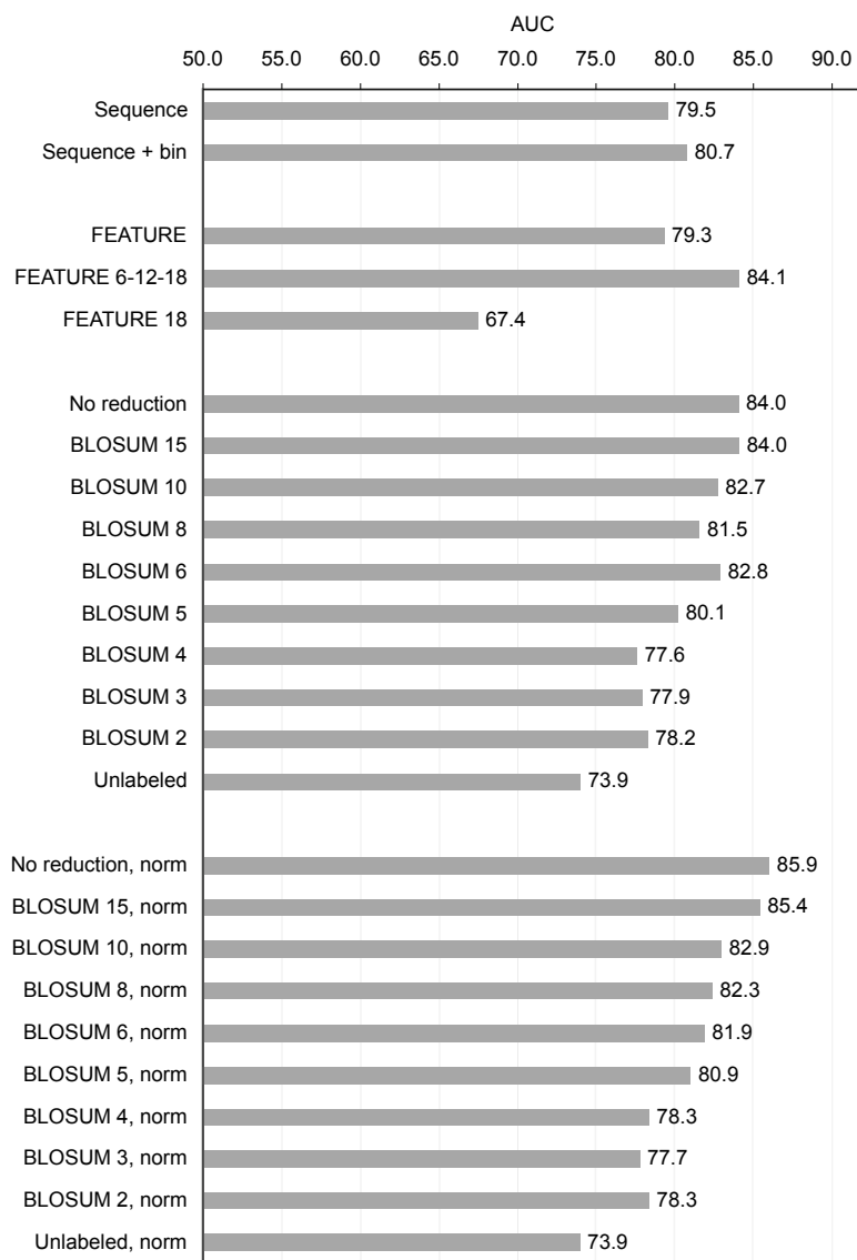
Supplementary Figure S9: Performance of all predictors on the CSA-Gly dataset.
