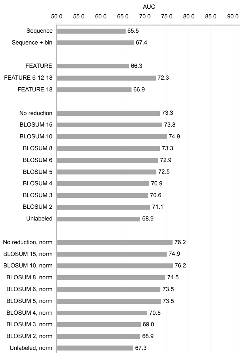
Supplementary Figure S3: Performance of all predictors on the CSA-Arg dataset.
