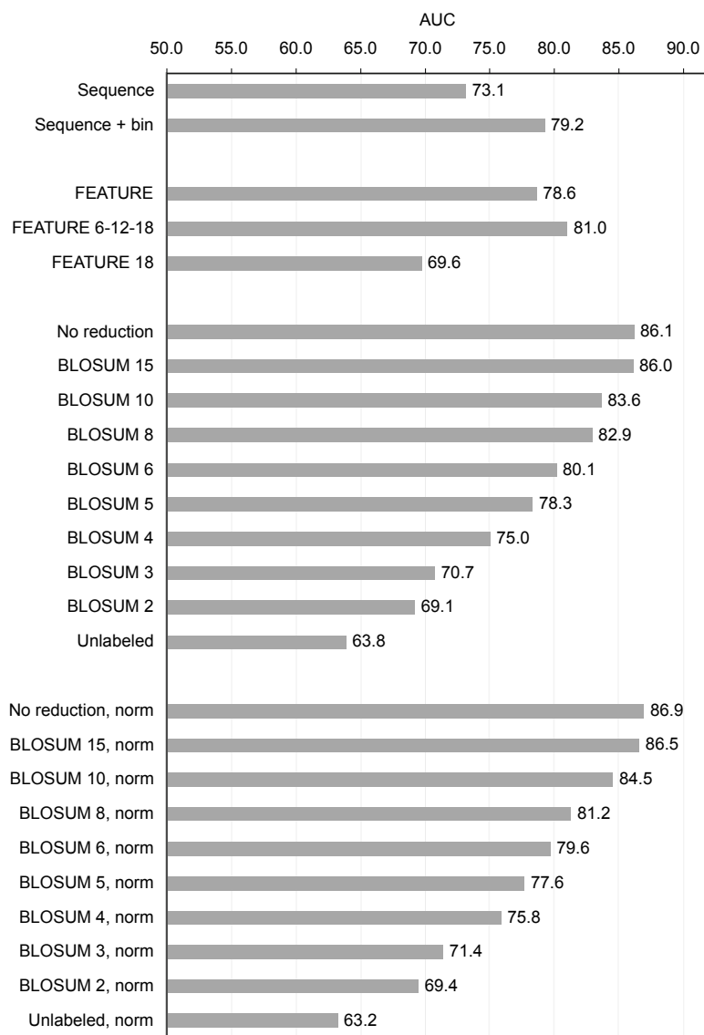
Supplementary Figure S6: Performance of all predictors on the CSA-Cys dataset.
