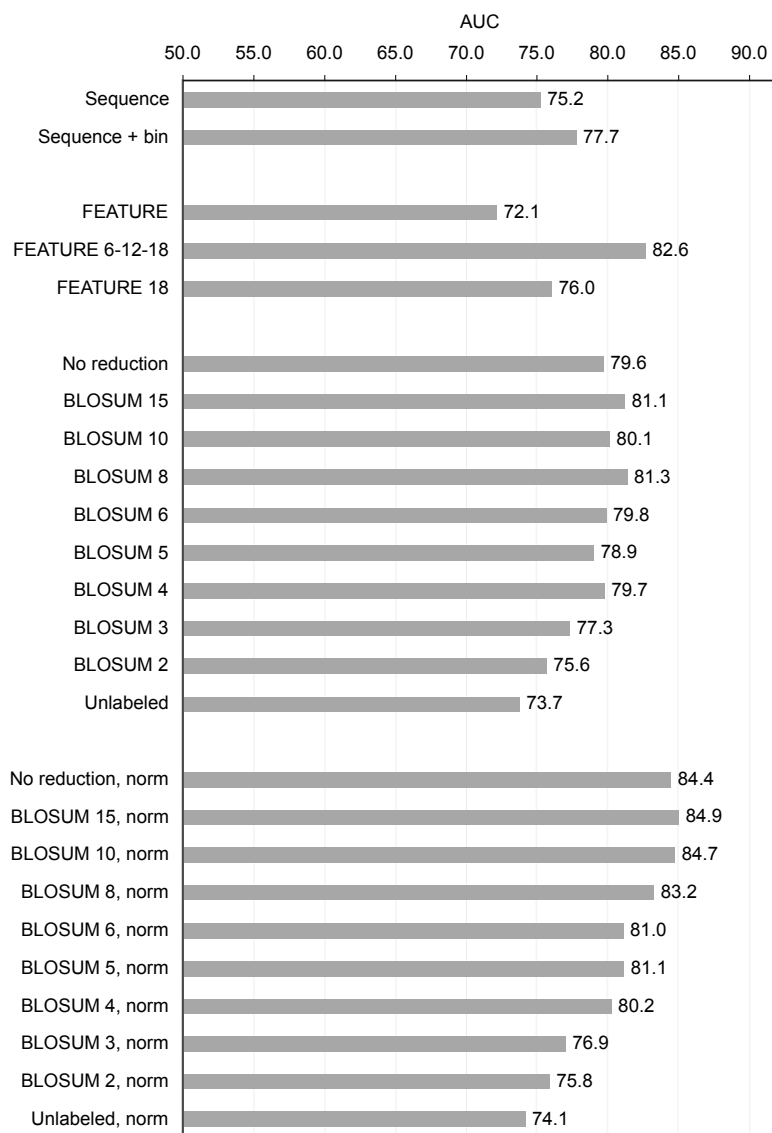
Supplementary Figure S4: Performance of all predictors on the CSA-Asn dataset.
